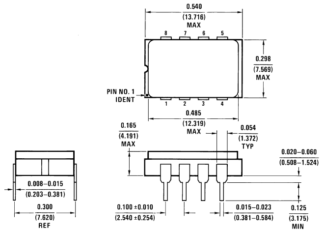
8-Pin Ceramic Sidebraced Dual-In-Line Package Order Number LM6142AMJ-QML NS Package Number D08C
