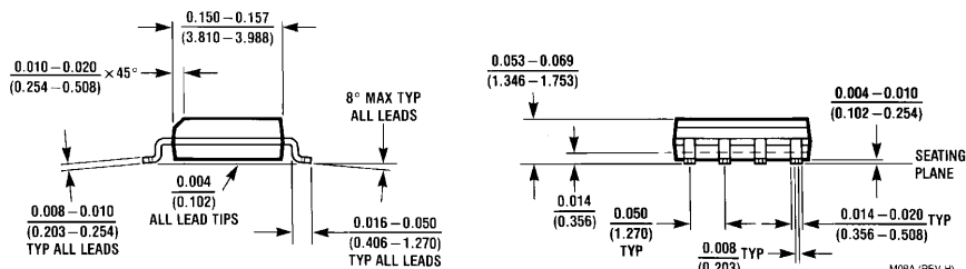
8-Pin Small Outline Package Order Number LM6142AIM or LM6142BIM NS Package Number M08A
